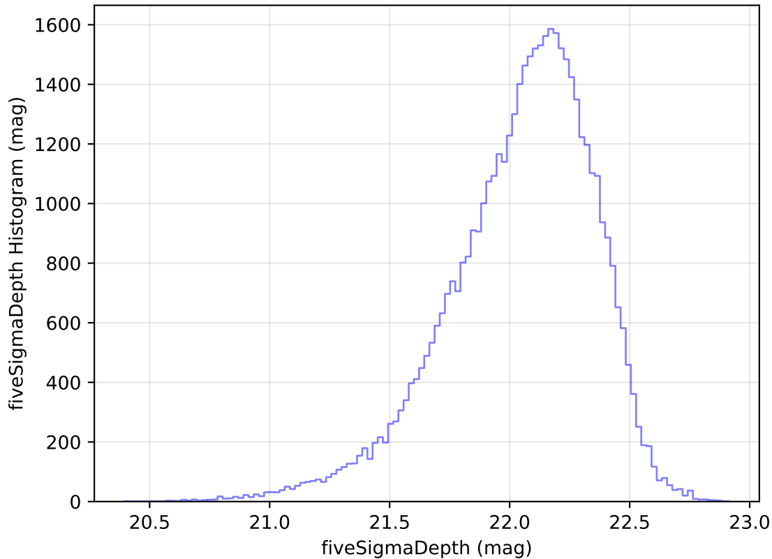
ddf_acor_sf20_lsf40_lsr10_v3.4_10yrs Yr 1 y band: fiveSigmaDepth Histogram
