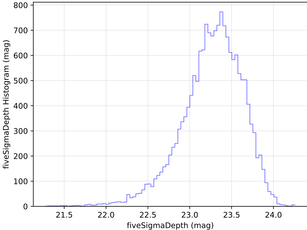
ddf_acor_sf20_lsf40_lsr10_v3.4_10yrs Yr 1 u band: fiveSigmaDepth Histogram
