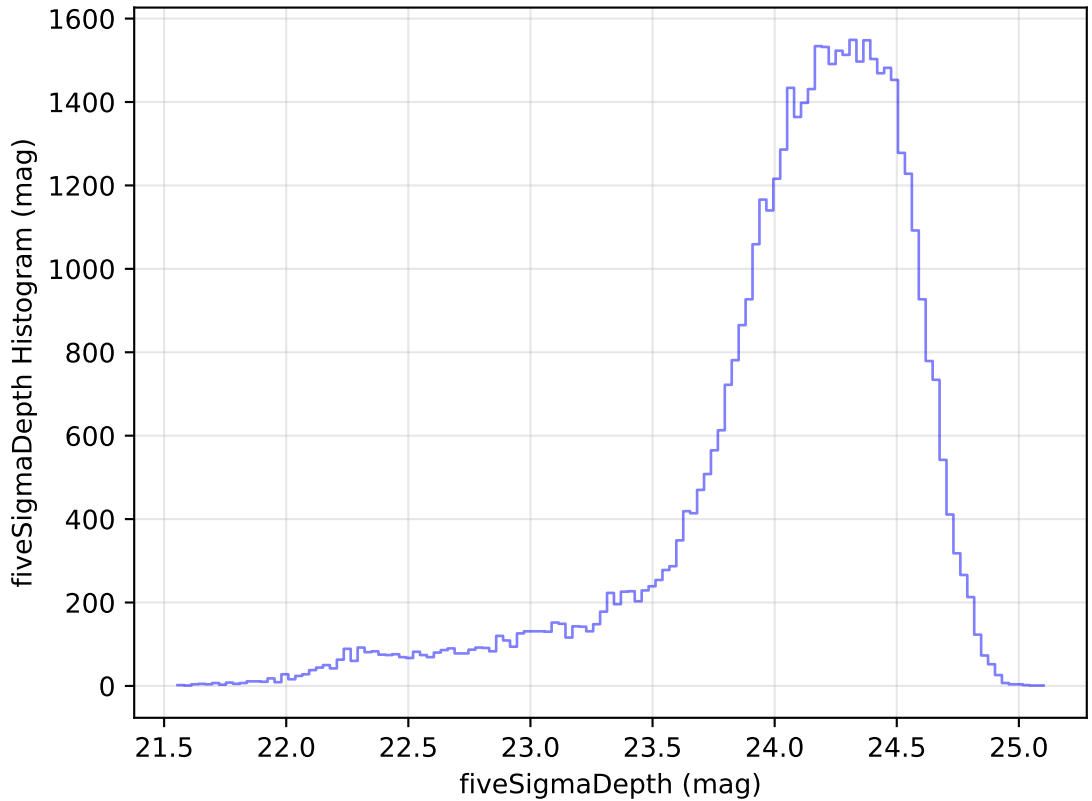
ddf_acor_sf20_lsf40_lsr10_v3.4_10yrs Yr 1 r band: fiveSigmaDepth Histogram
