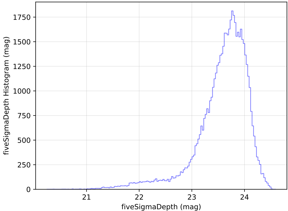
ddf_acor_sf20_lsf40_lsr10_v3.4_10yrs Yr 1 i band: fiveSigmaDepth Histogram
