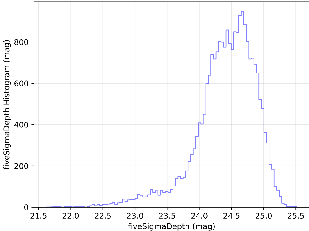
ddf_acor_sf20_lsf40_lsr10_v3.4_10yrs Yr 1 g band: fiveSigmaDepth Histogram
