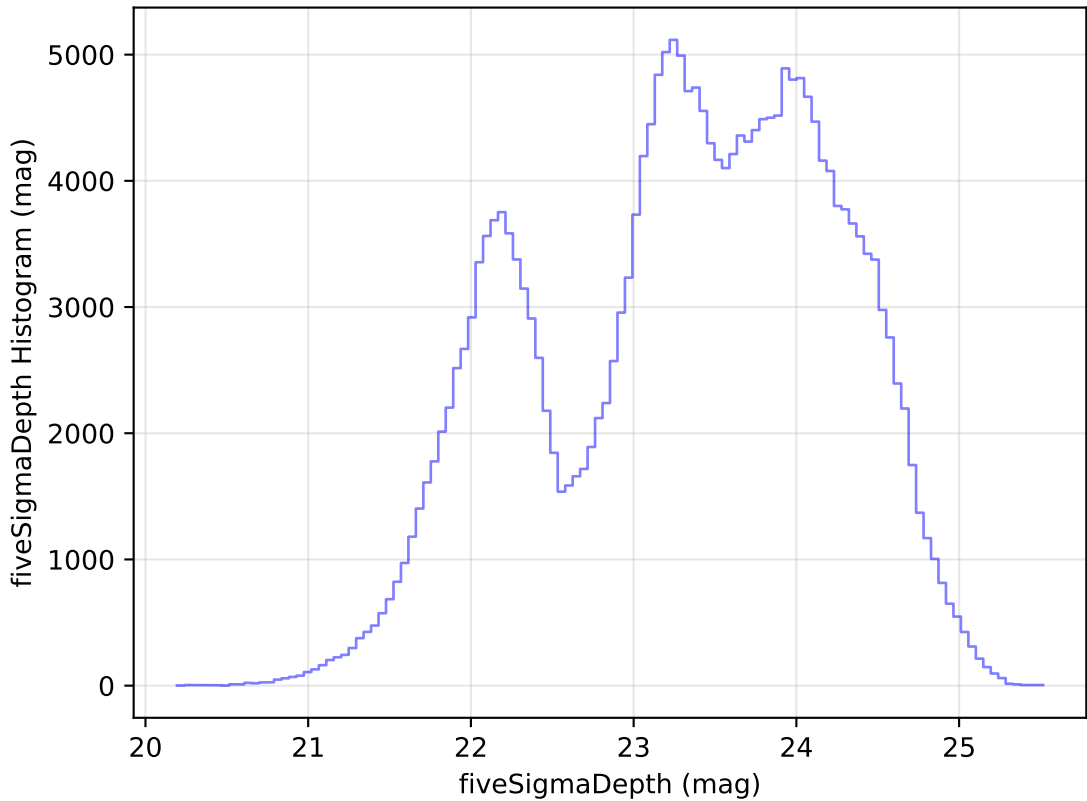
ddf_acor_sf20_lsf40_lsr10_v3.4_10yrs Yr 1 all bands: fiveSigmaDepth Histogram
