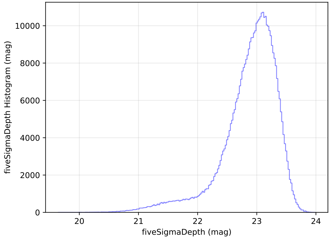
ddf_acor_sf20_lsf40_lsr10_v3.4_10yrs WFD z band: fiveSigmaDepth Histogram
