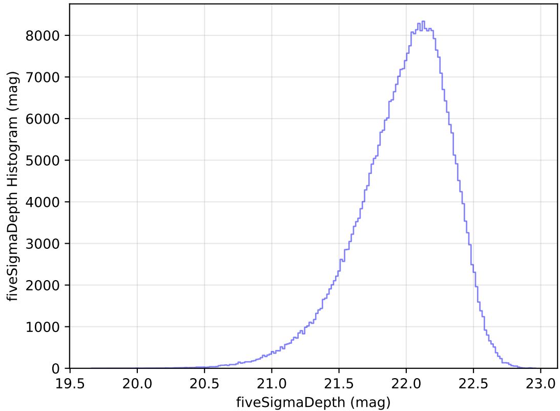
ddf_acor_sf20_lsf40_lsr10_v3.4_10yrs WFD y band: fiveSigmaDepth Histogram
