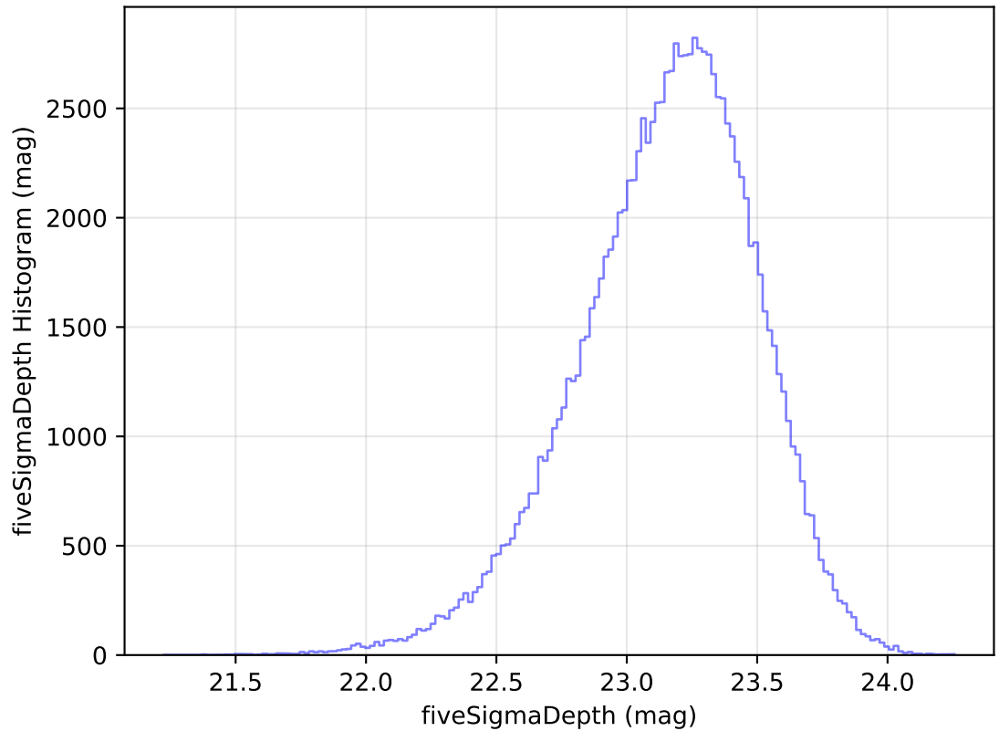
ddf_acor_sf20_lsf40_lsr10_v3.4_10yrs WFD u band: fiveSigmaDepth Histogram
