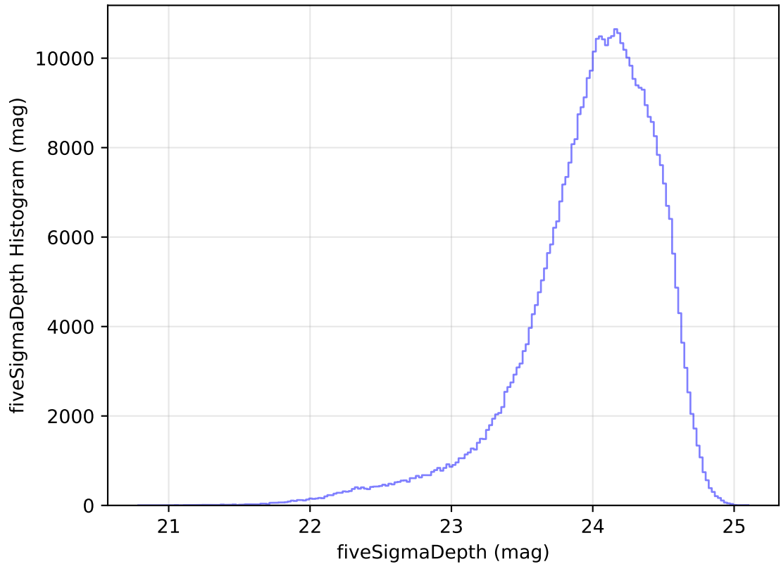
ddf_acor_sf20_lsf40_lsr10_v3.4_10yrs WFD r band: fiveSigmaDepth Histogram
