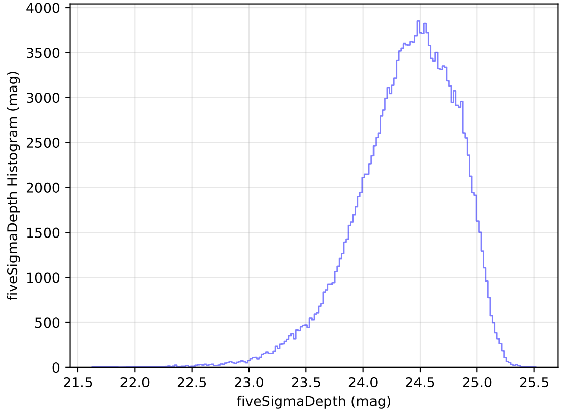
ddf_acor_sf20_lsf40_lsr10_v3.4_10yrs WFD g band: fiveSigmaDepth Histogram
