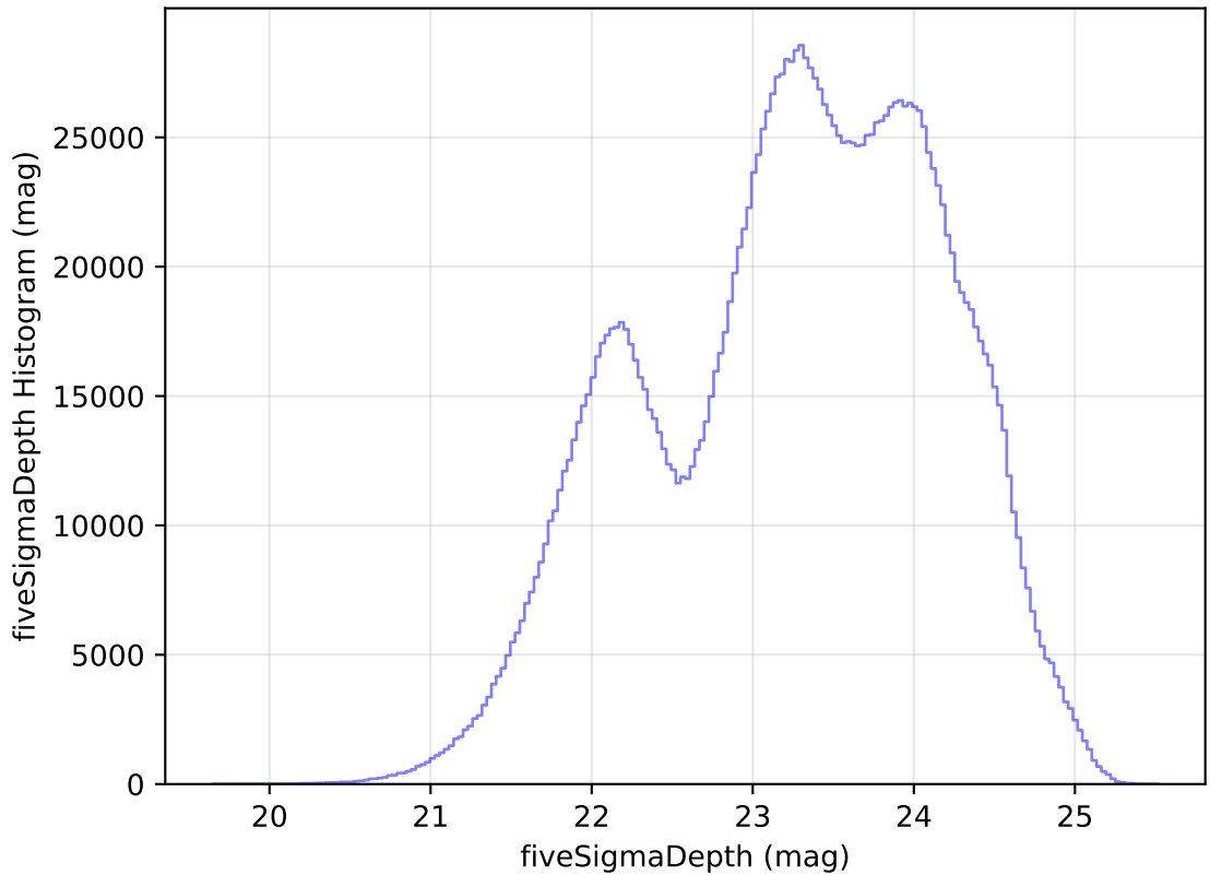
ddf_acor_sf20_lsf40_lsr10_v3.4_10yrs WFD all bands: fiveSigmaDepth Histogram
