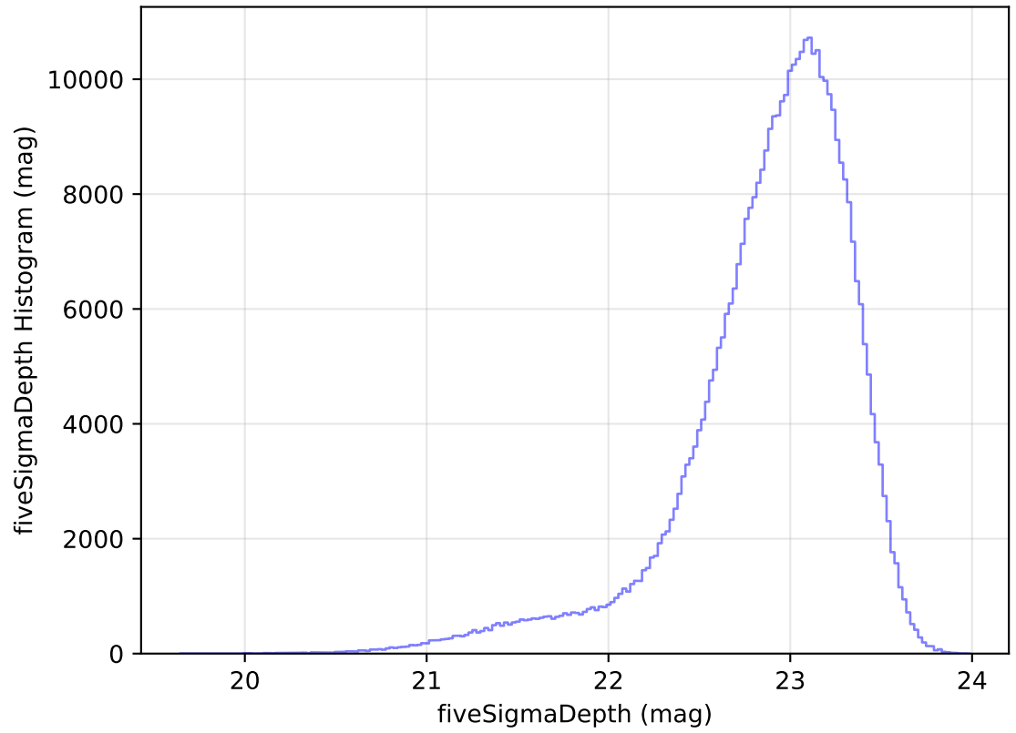
ddf_acor_sf20_lsf40_lsr10_v3.4_10yrs All sky z band: fiveSigmaDepth Histogram
