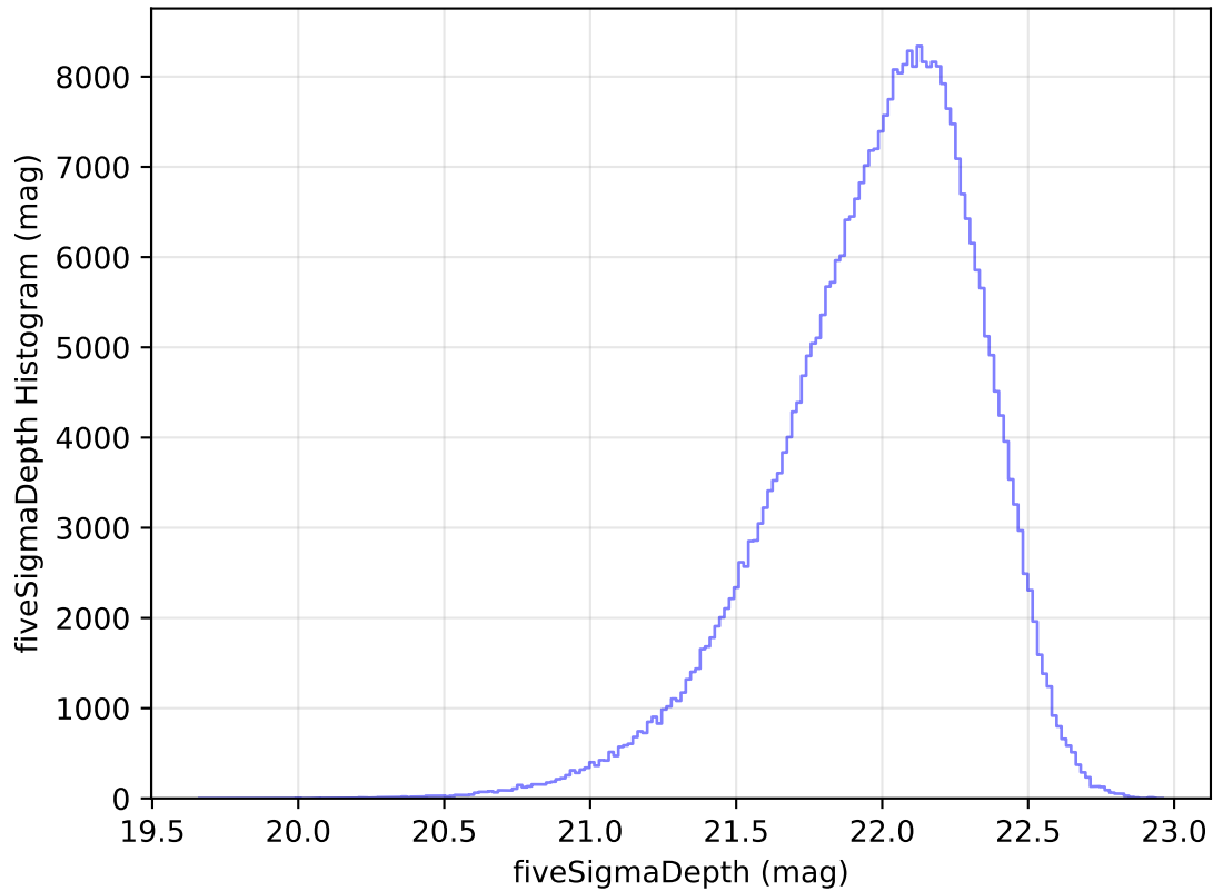
ddf_acor_sf20_lsf40_lsr10_v3.4_10yrs All sky y band: fiveSigmaDepth Histogram
