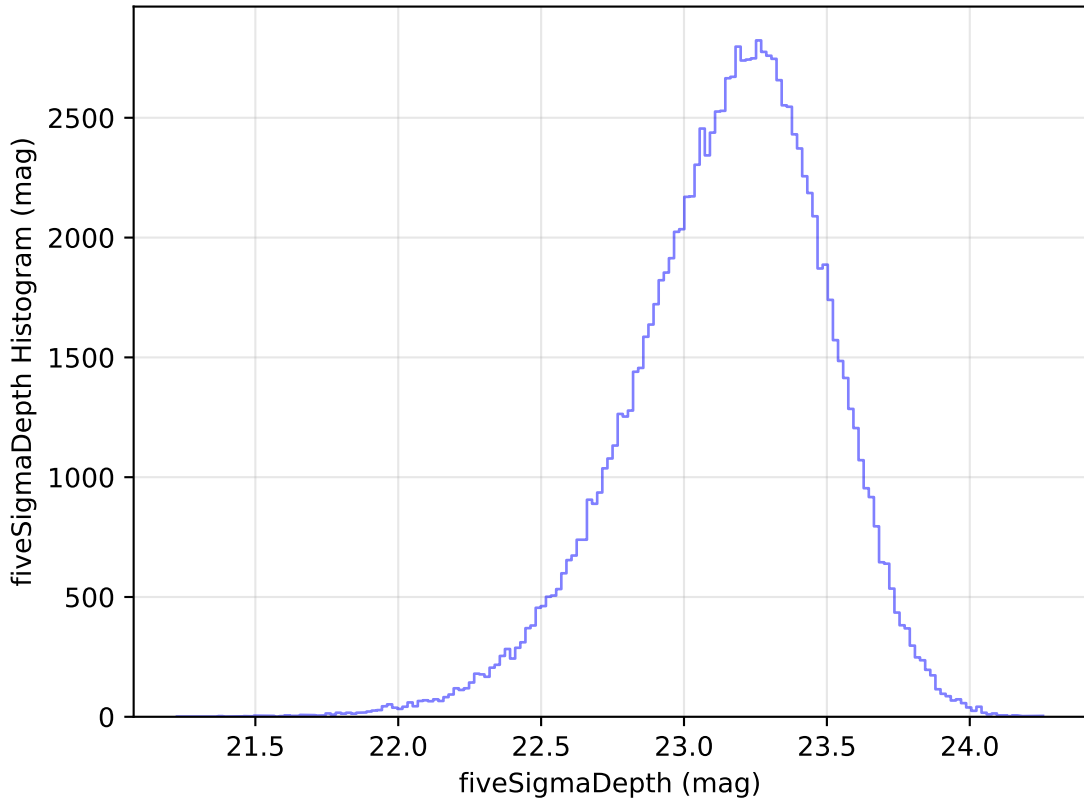
ddf_acor_sf20_lsf40_lsr10_v3.4_10yrs All sky u band: fiveSigmaDepth Histogram
