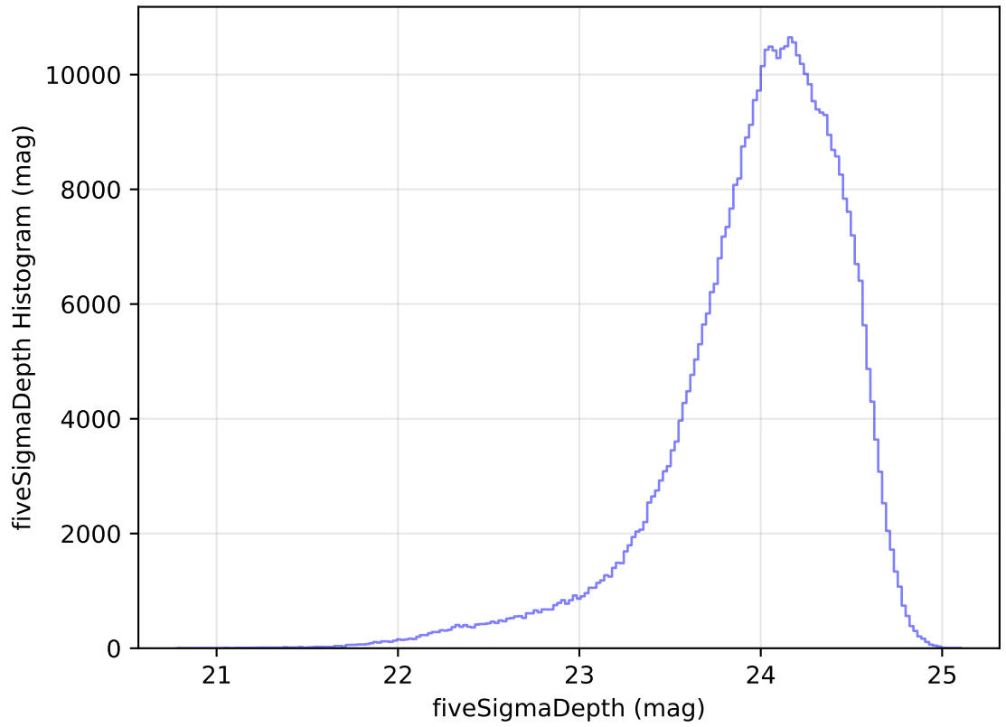
ddf_acor_sf20_lsf40_lsr10_v3.4_10yrs All sky r band: fiveSigmaDepth Histogram
