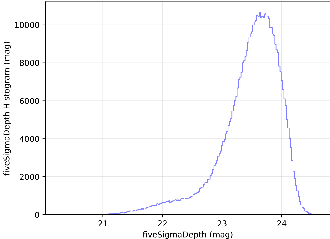
ddf_acor_sf20_lsf40_lsr10_v3.4_10yrs All sky i band: fiveSigmaDepth Histogram
