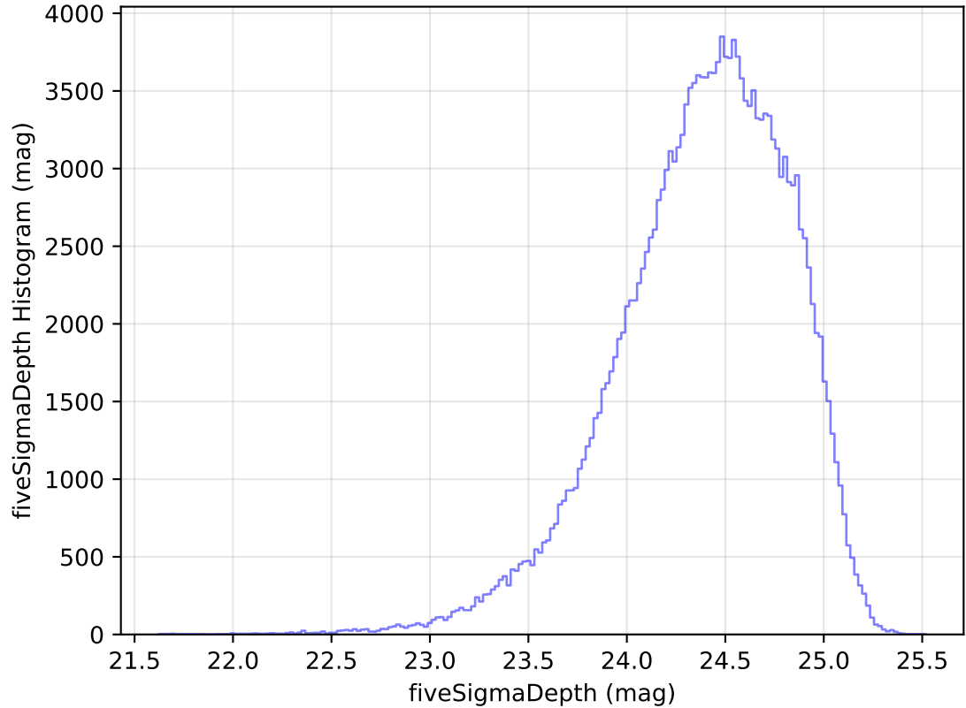
ddf_acor_sf20_lsf40_lsr10_v3.4_10yrs All sky g band: fiveSigmaDepth Histogram
