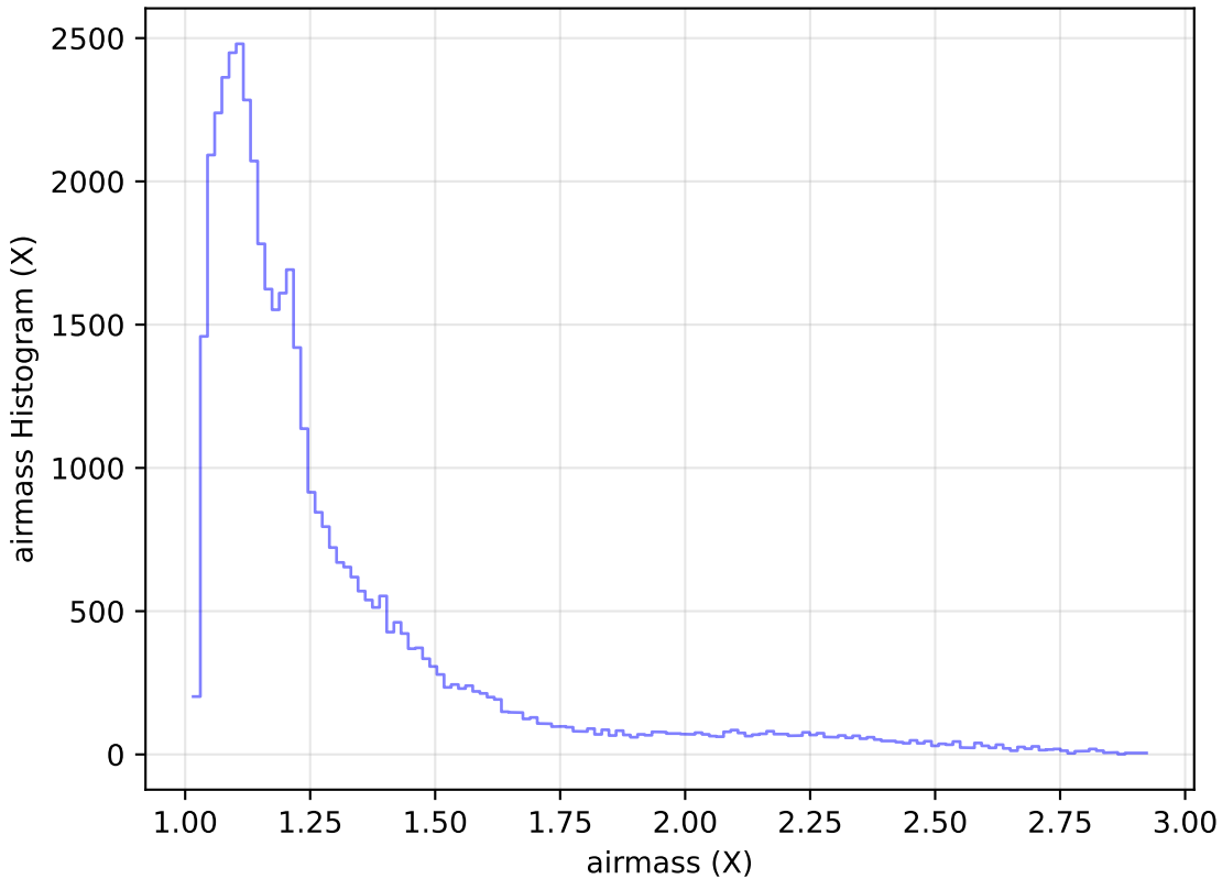
ddf_acor_sf20_lsf40_lsr10_v3.4_10yrs Yr 1 z band: airmass Histogram
