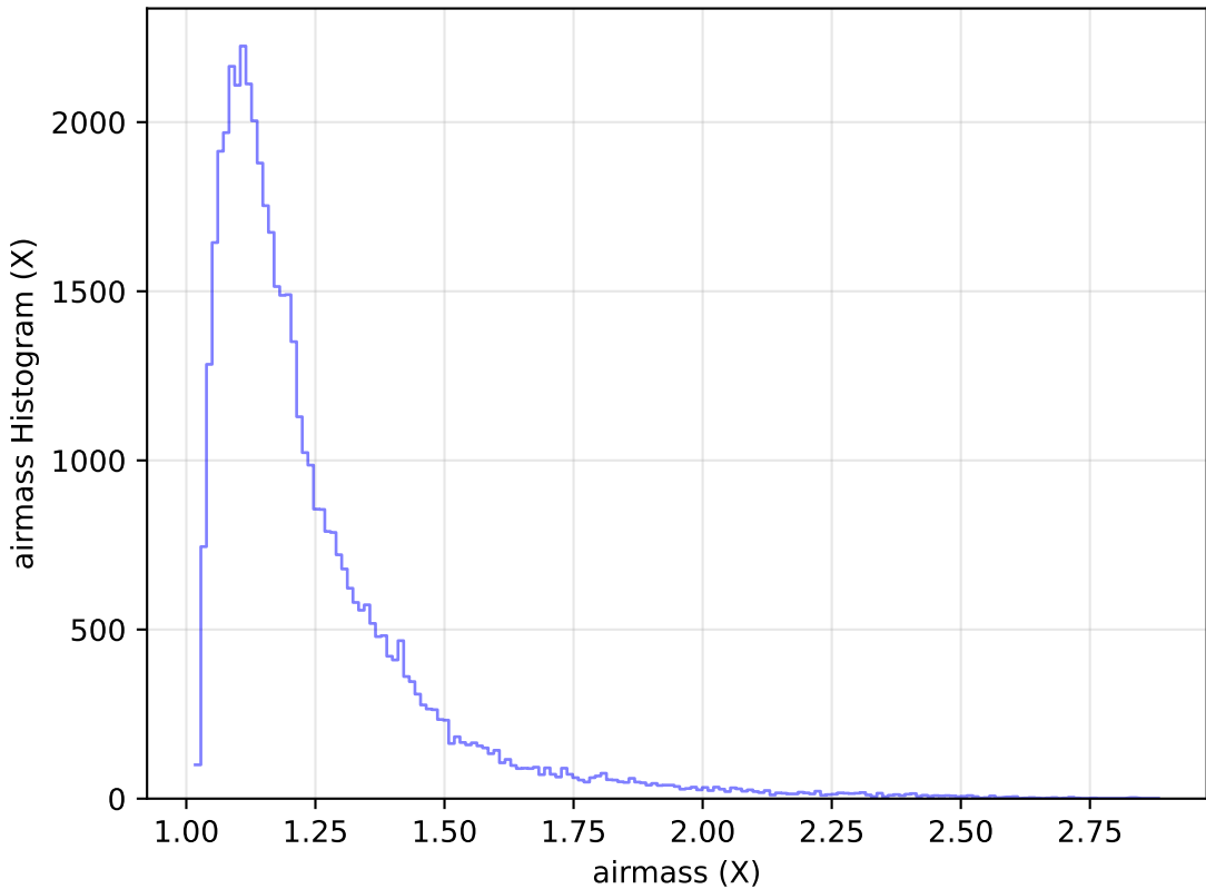
ddf_acor_sf20_lsf40_lsr10_v3.4_10yrs Yr 1 y band: airmass Histogram
