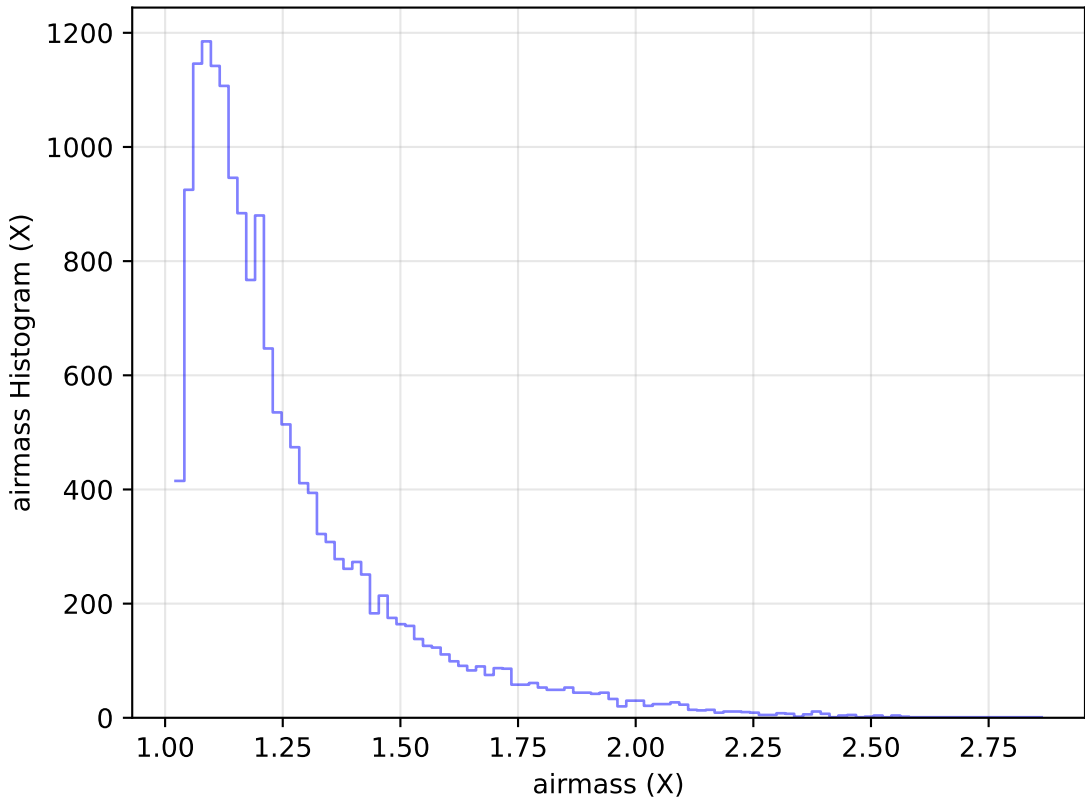
ddf_acor_sf20_lsf40_lsr10_v3.4_10yrs Yr 1 u band: airmass Histogram
