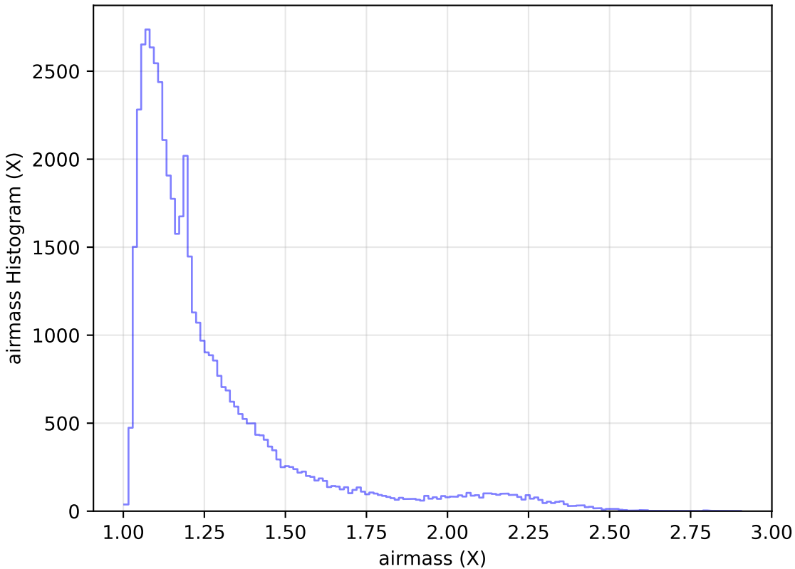
ddf_acor_sf20_Isf40_Isr10_v3.4_10yrs Yr 1 r band: airmass Histogram
