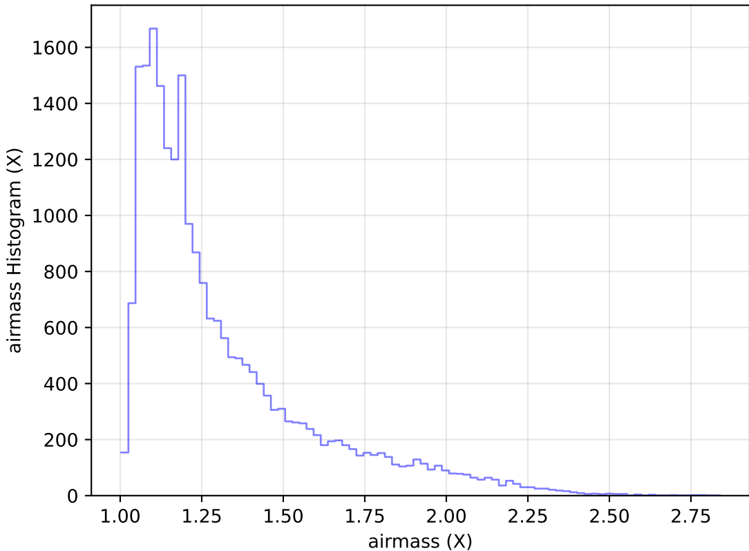
ddf_acor_sf20_lsf40_lsr10_v3.4_10yrs Yr 1 g band: airmass Histogram
