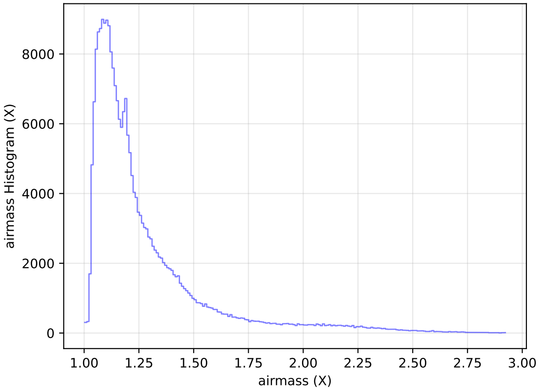
ddf_acor_sf20_lsf40_lsr10_v3.4_10yrs Yr 1 all bands: airmass Histogram
