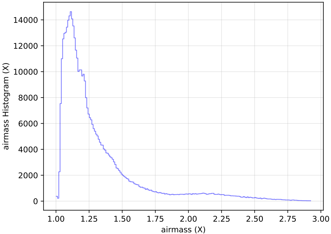
ddf_acor_sf20_lsf40_lsr10_v3.4_10yrs WFD z band: airmass Histogram
