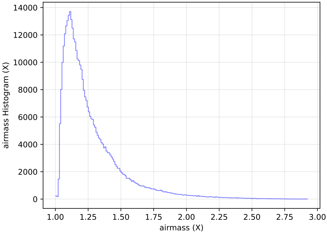
ddf_acor_sf20_lsf40_lsr10_v3.4_10yrs WFD y band: airmass Histogram
