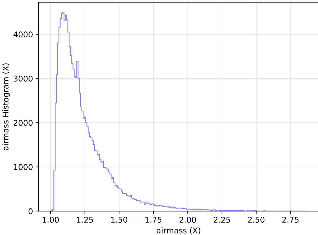
ddf_acor_sf20_lsf40_lsr10_v3.4_10yrs WFD u band: airmass Histogram
