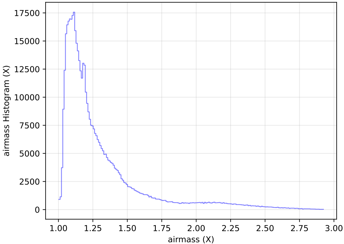
ddf_acor_sf20_lsf40_lsr10_v3.4_10yrs WFD i band: airmass Histogram
