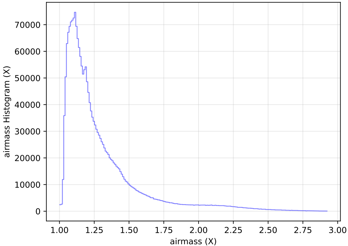
ddf_acor_sf20_lsf40_lsr10_v3.4_10yrs WFD all bands: airmass Histogram
