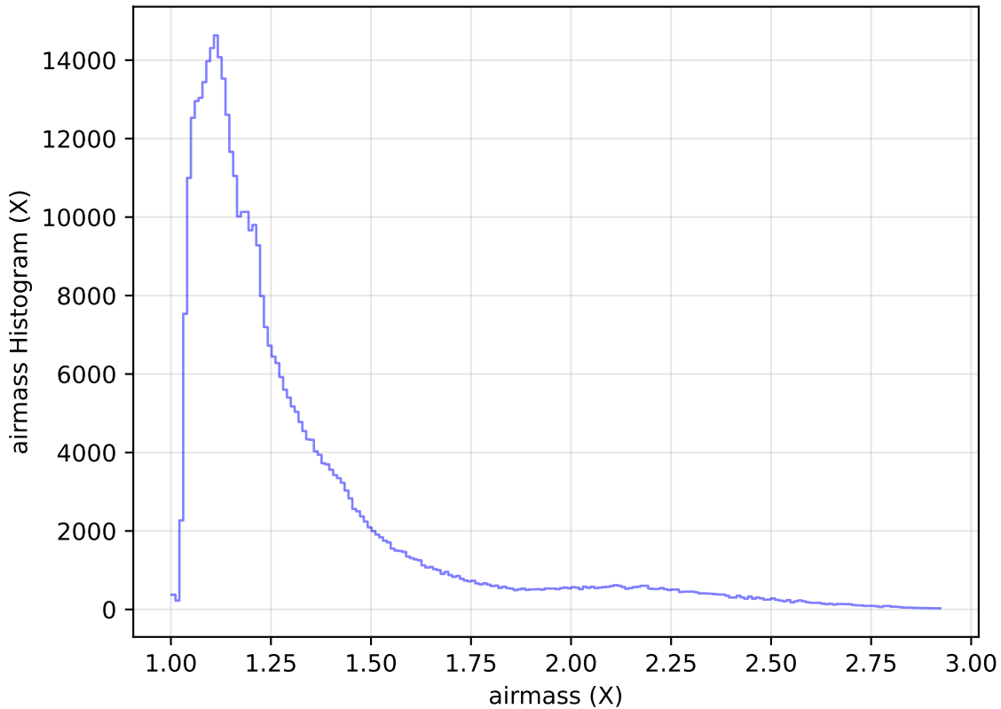
ddf_acor_sf20_lsf40_lsr10_v3.4_10yrs All sky z band: airmass Histogram
