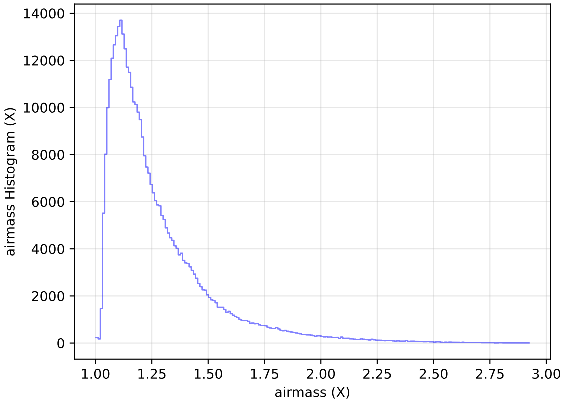
ddf_acor_sf20_lsf40_lsr10_v3.4_10yrs All sky y band: airmass Histogram
