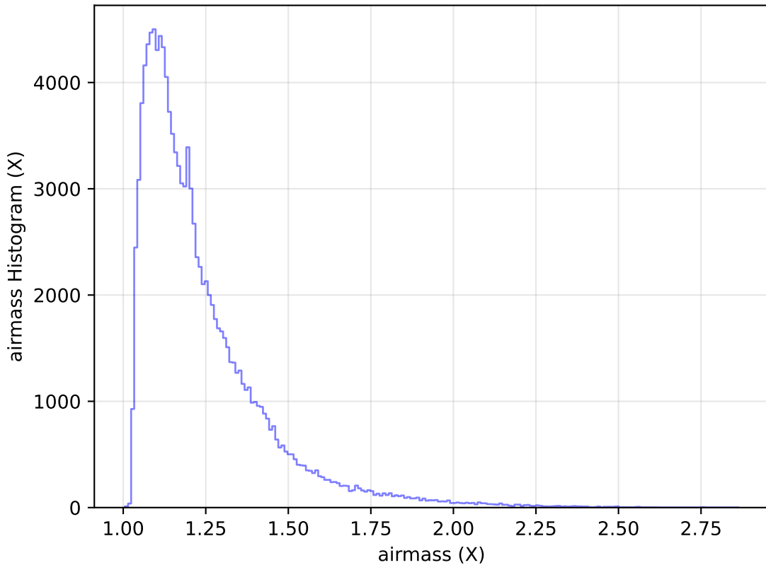
ddf_acor_sf20_lsf40_lsr10_v3.4_10yrs All sky u band: airmass Histogram
