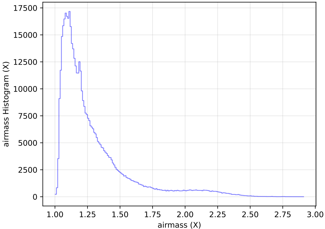
ddf_acor_sf20_lsf40_lsr10_v3.4_10yrs All sky r band: airmass Histogram
