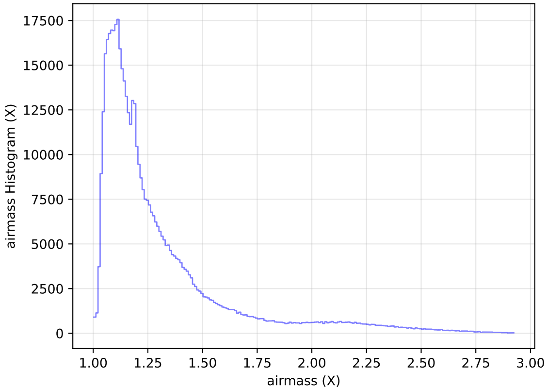
ddf_acor_sf20_lsf40_lsr10_v3.4_10yrs All sky i band: airmass Histogram
