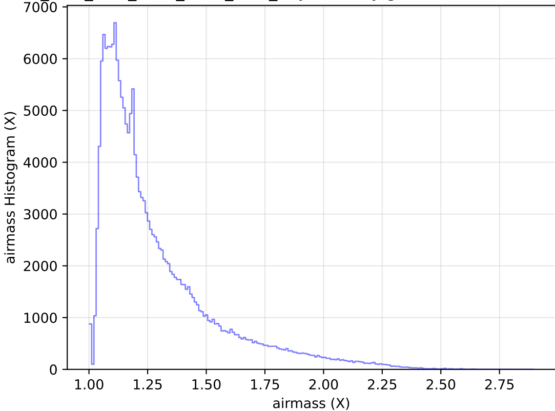
ddf_acor_sf20_lsf40_lsr10_v3.4_10yrs All sky g band: airmass Histogram
