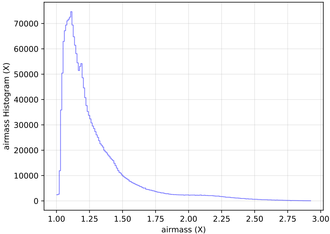
ddf_acor_sf20_lsf40_lsr10_v3.4_10yrs All sky all bands: airmass Histogram
