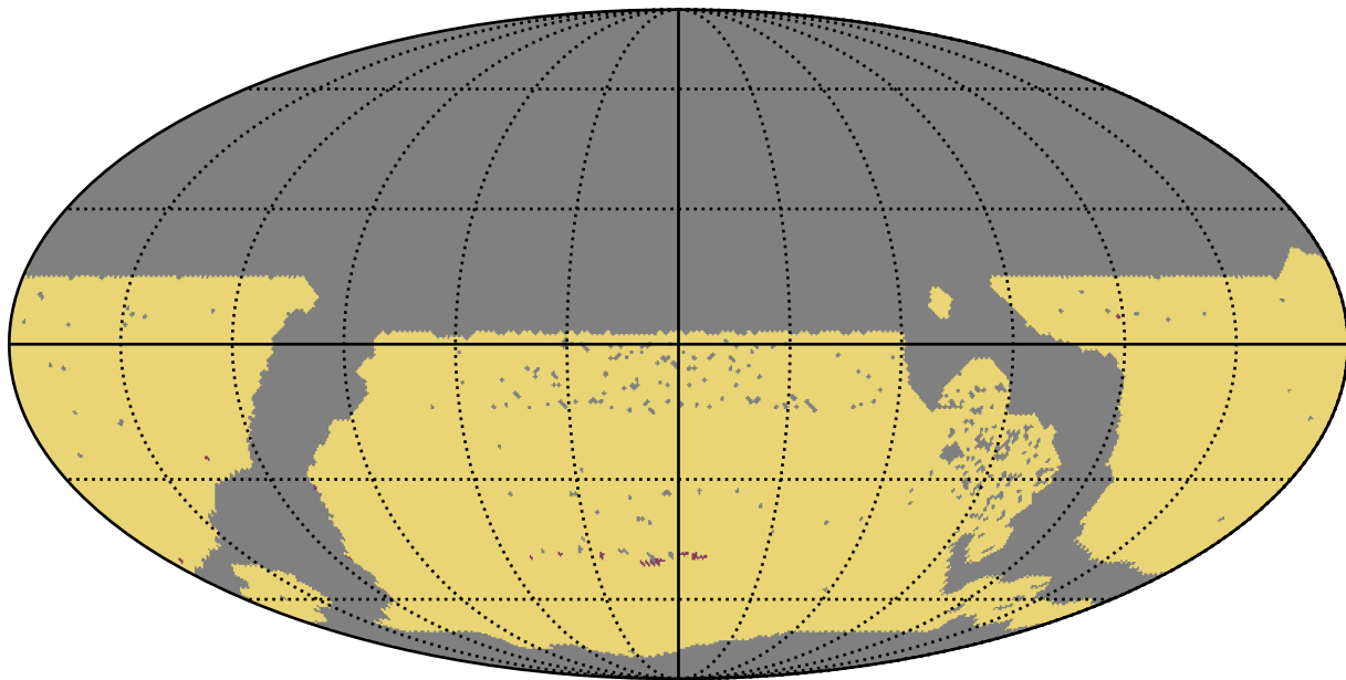
ddf_acor_sf20_lsf40_lsr10_v3.4_10yrs WFD: RapidRevisits
