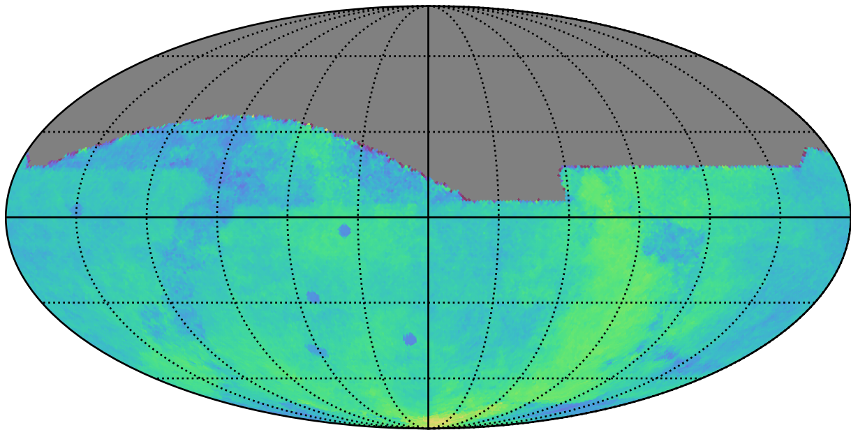
ddf_acor_sf20_lsf40_lsr10_v3.4_10yrs All sky: Parallax Coverage @ 24.0
