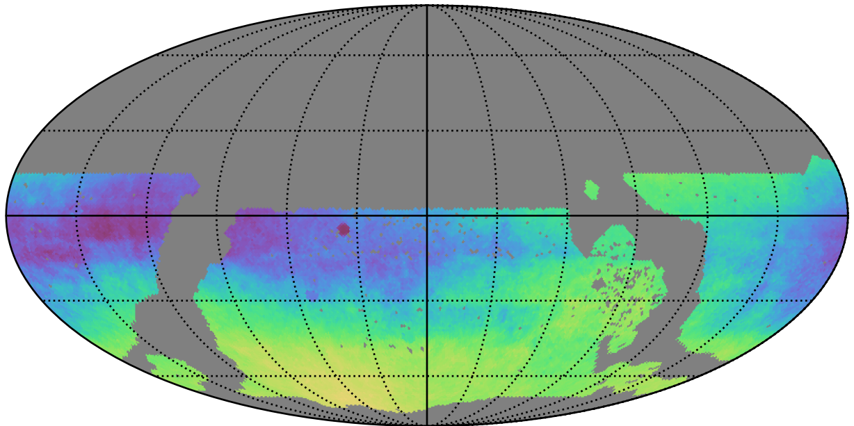
ddf_acor_sf20_lsf40_lsr10_v3.4_10yrs WFD: Parallax-DCR degeneracy @ 24.0
