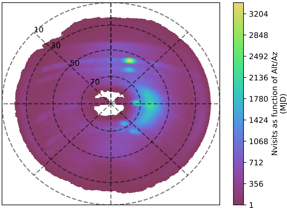
ddf_acor_sf20_lsf40_lsr10_v3.4_10yrs z band: Nvisits as function of Alt/Az
