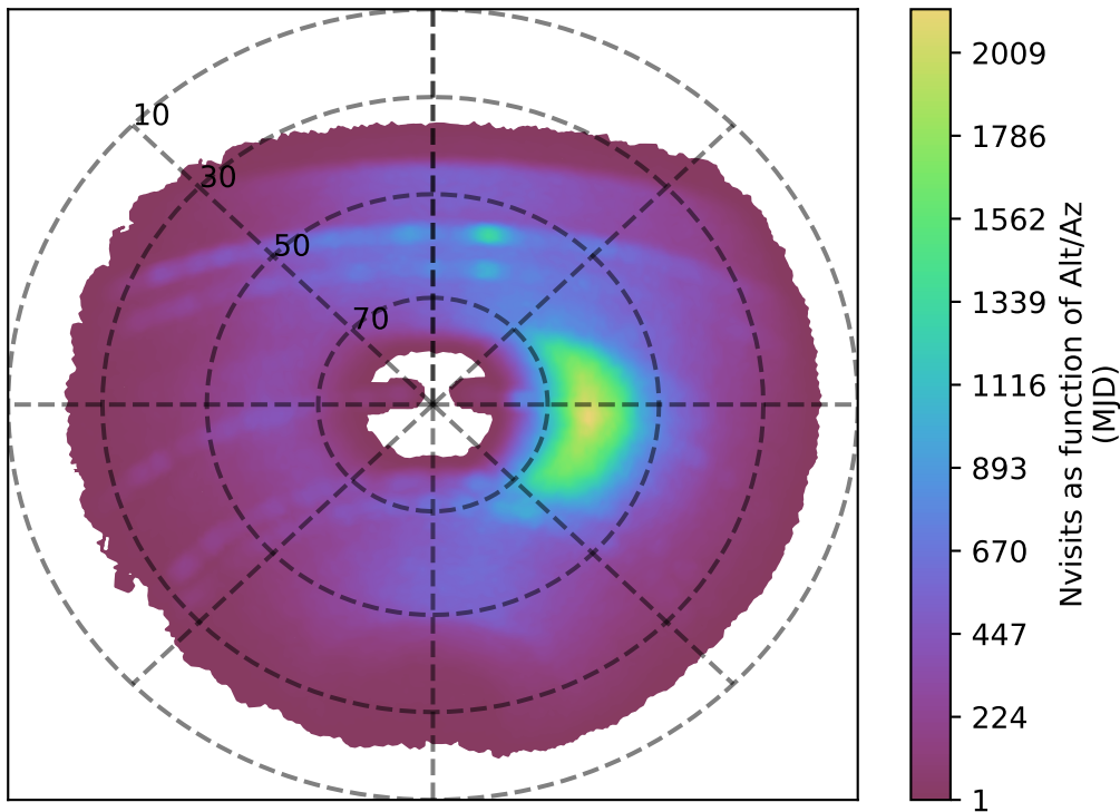
ddf_acor_sf20_lsf40_lsr10_v3.4_10yrs y band: Nvisits as function of Alt/Az
