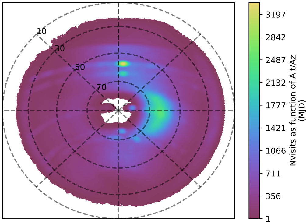
ddf_acor_sf20_lsf40_lsr10_v3.4_10yrs i band: Nvisits as function of Alt/Az
