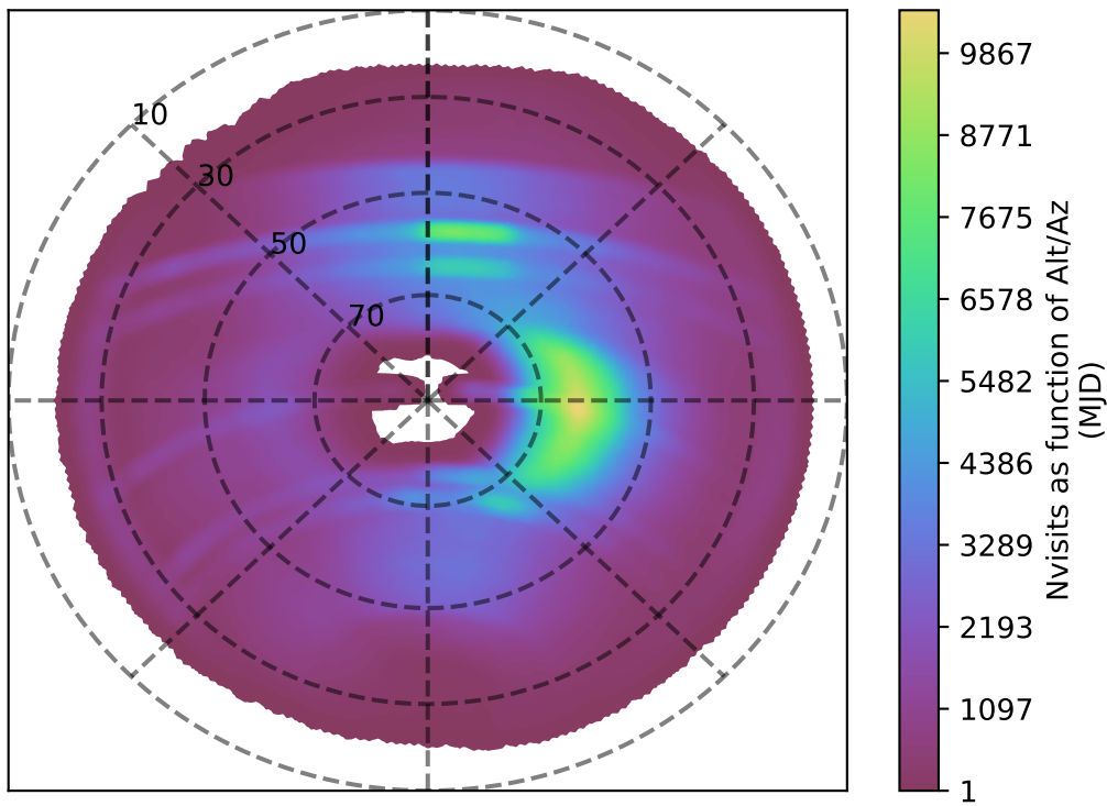
ddf_acor_sf20_lsf40_lsr10_v3.4_10yrs all bands: Nvisits as function of Alt/Az
