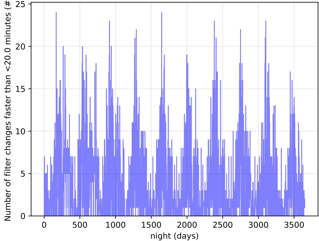
ddf_acor_sf20_Isf40_Isr10_v3.4_10yrs Per Night: Number of filter changes faster than <20.0 minutes
