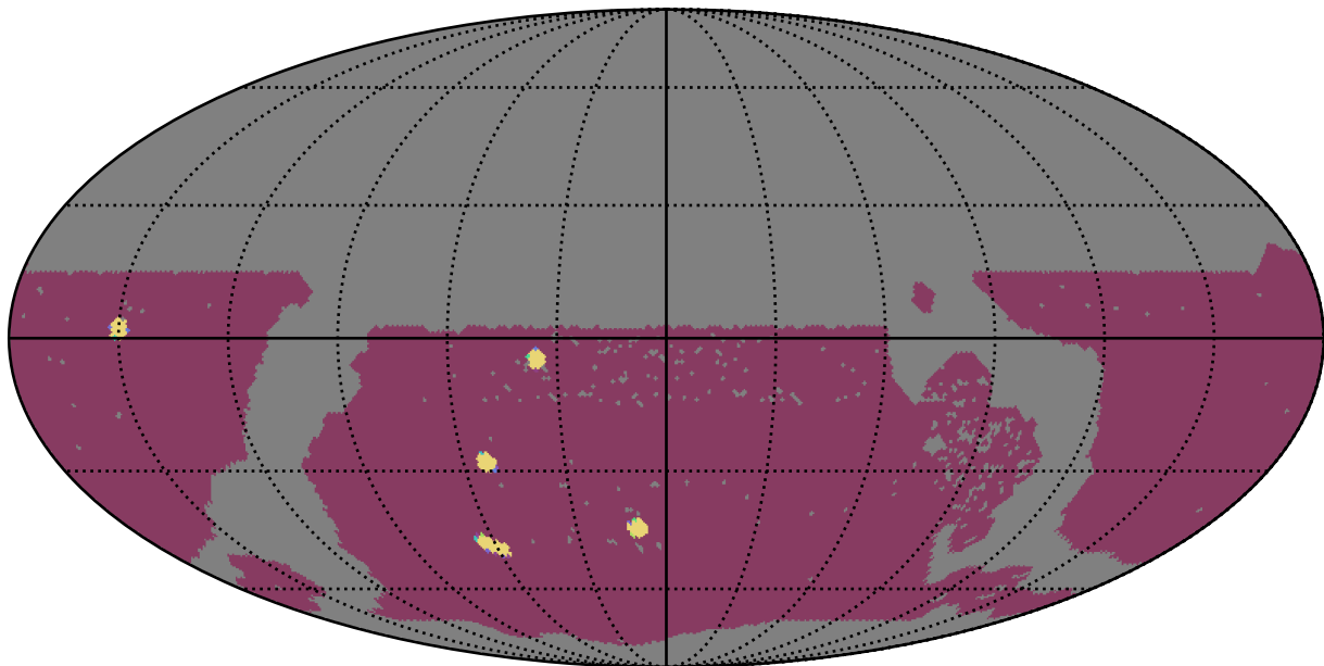
ddf_acor_sf20_lsf40_lsr10_v3.4_10yrs WFD: NumberOfQuickRevisits
