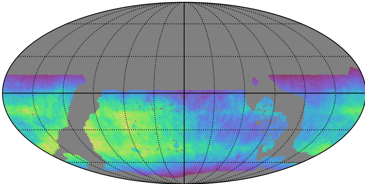
ddf_acor_sf20_lsf40_lsr10_v3.4_10yrs WFD r band: Normalized Teff
