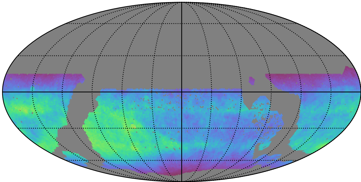
ddf_acor_sf20_lsf40_lsr10_v3.4_10yrs WFD i band: Normalized Teff
