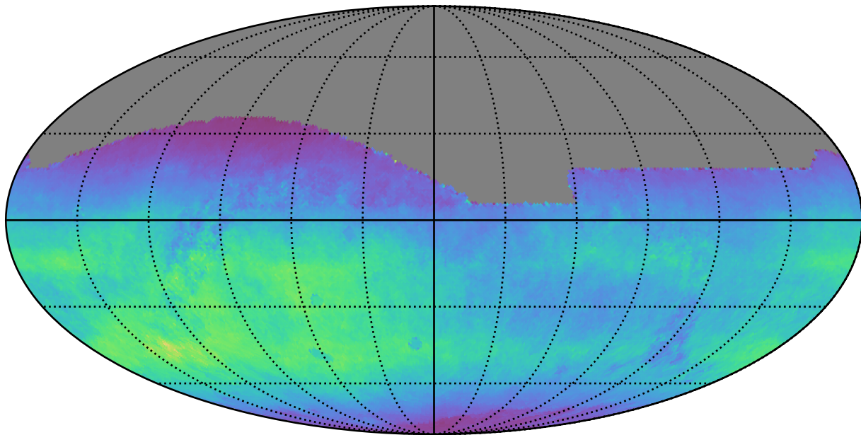
ddf_acor_sf20_lsf40_lsr10_v3.4_10yrs All sky r band: Normalized Teff
