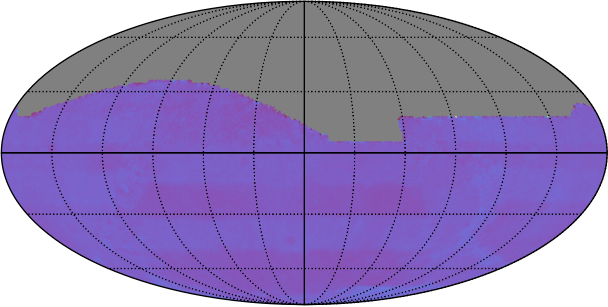
ddf_acor_sf20_lsf40_lsr10_v3.4_10yrs All sky: Normalized Proper Motion Uncert @ 24.0
