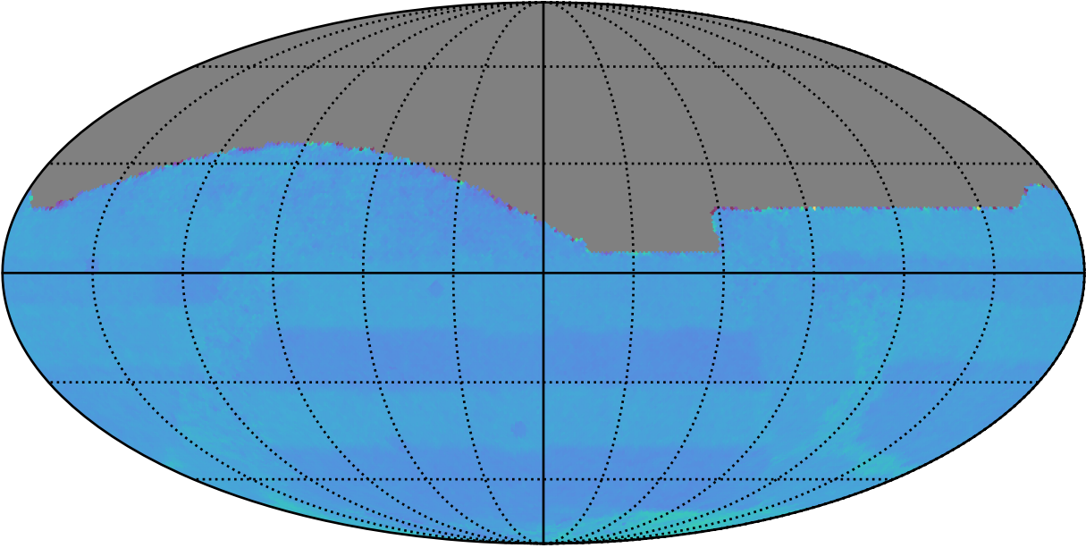
ddf_acor_sf20_lsf40_lsr10_v3.4_10yrs All sky: Normalized Proper Motion Uncert @ 20.5
